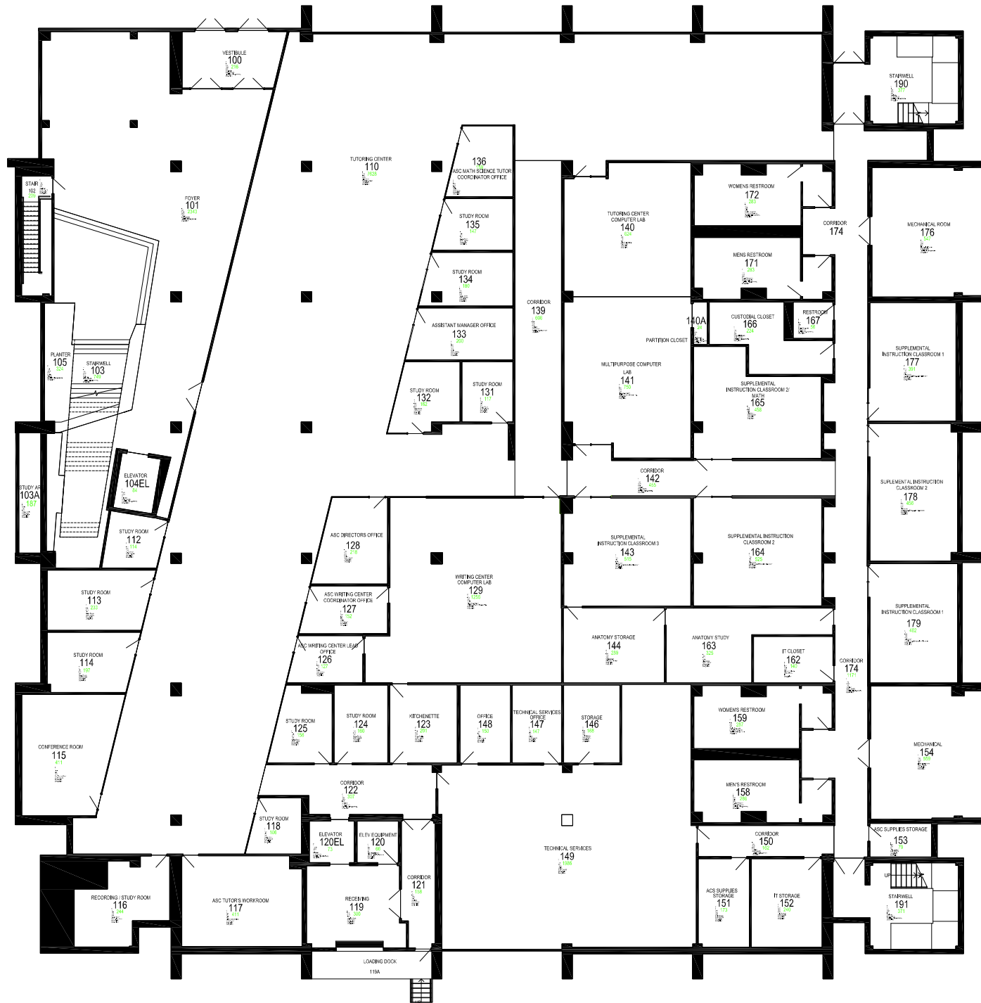
Building F - Level 1
